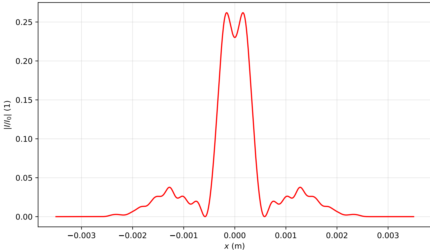
Intensity profile I(x, y = 0, z = 3.344)/I_0 , P_{in}=8.0P_{cr} , artificial time
